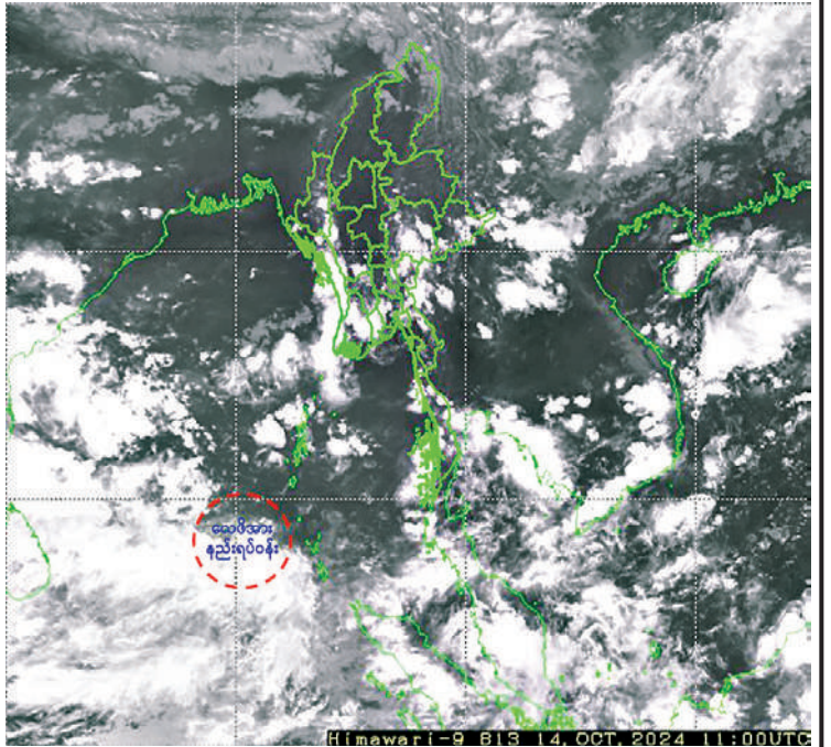
Himawari-9 615 14, OCT, 2024 11:00UTC
